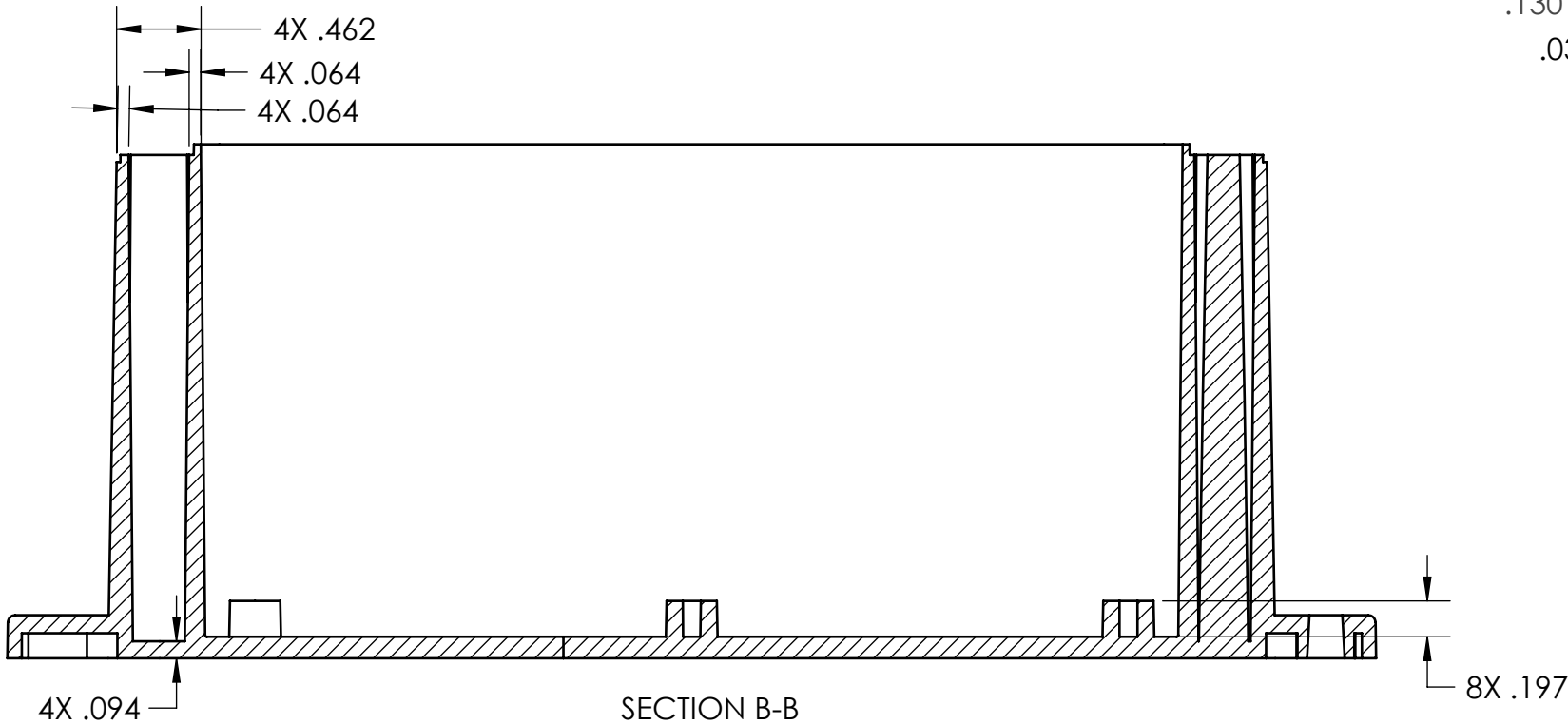
SECTION B-B
