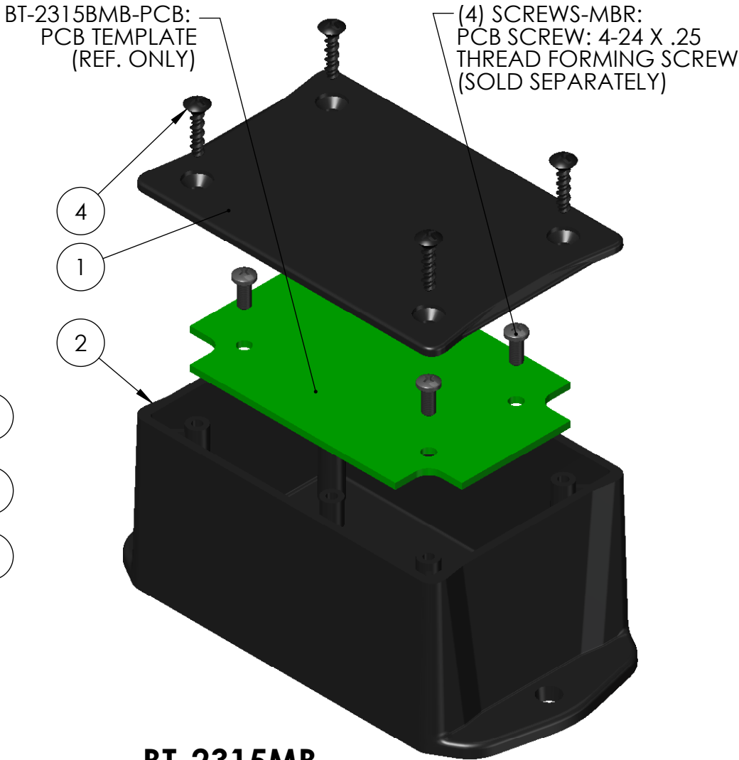
BT-2315MB BT SERIES ASSEMBLY, BLACK, WITH MOUNTING BOSSES FLAME RATING: UL94V-0
