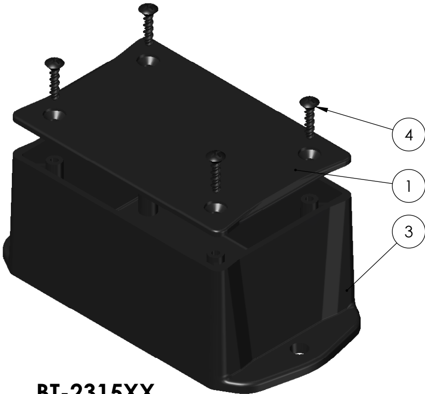
BT-2315XX BT SERIES ASSEMBLY, BLACK, WITHOUT MOUNTING BOSSES FLAME RATING: UL94V-0
