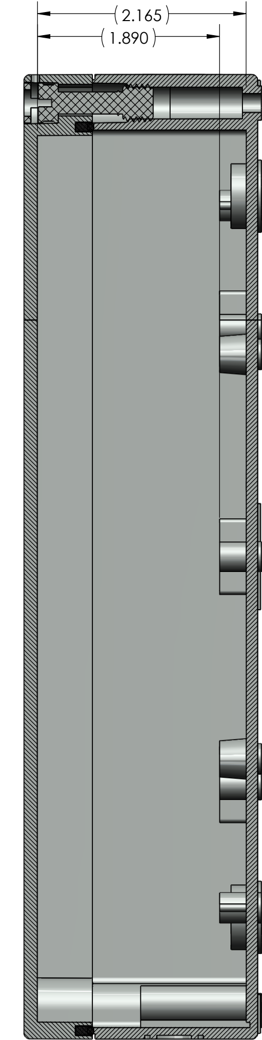
SECTION B-B
