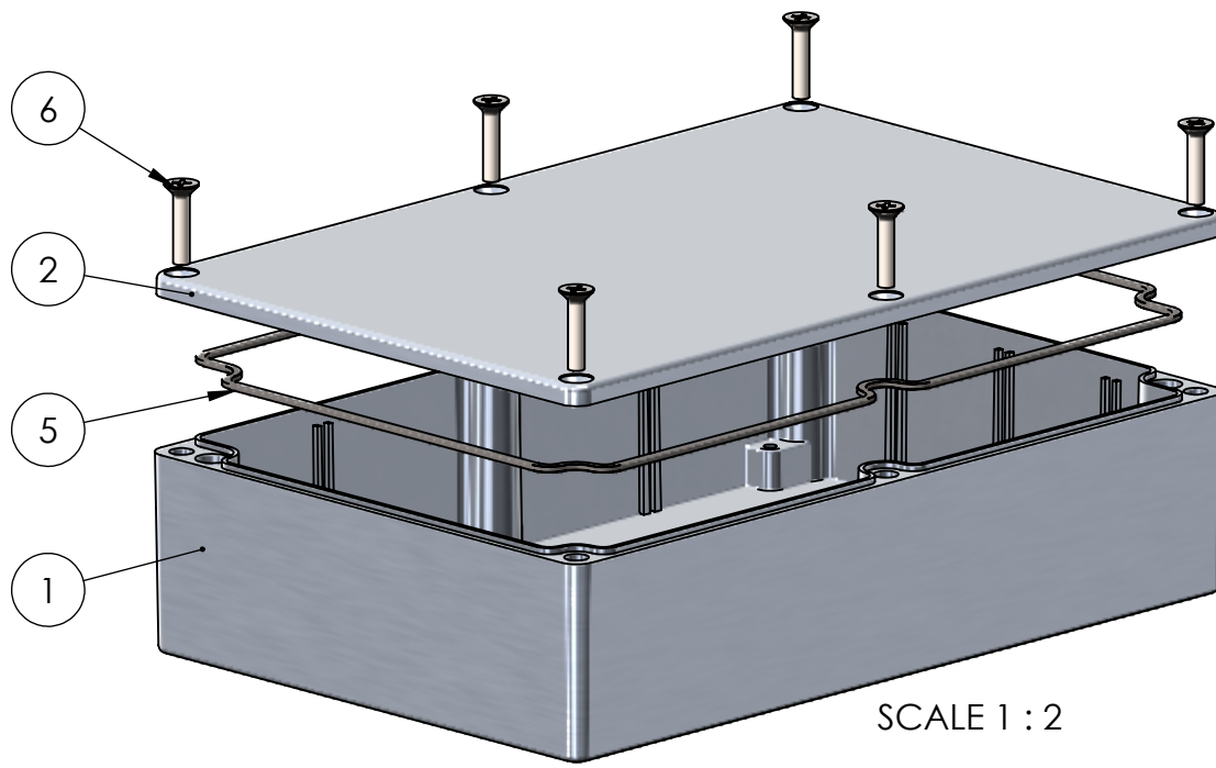
PART NUMBER: AN-07P-01
