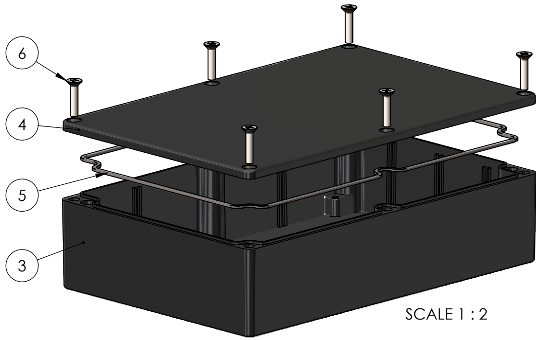
PART NUMBER: AN-07P-02
