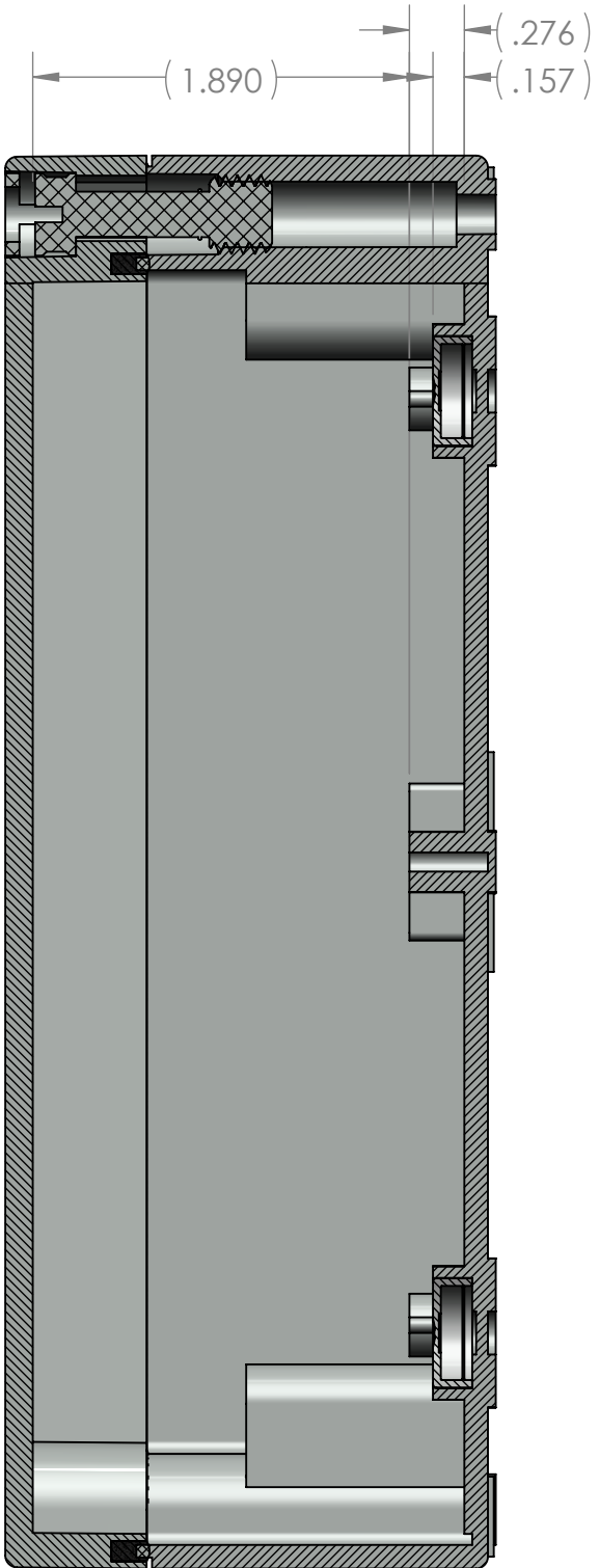
SECTION B-B
