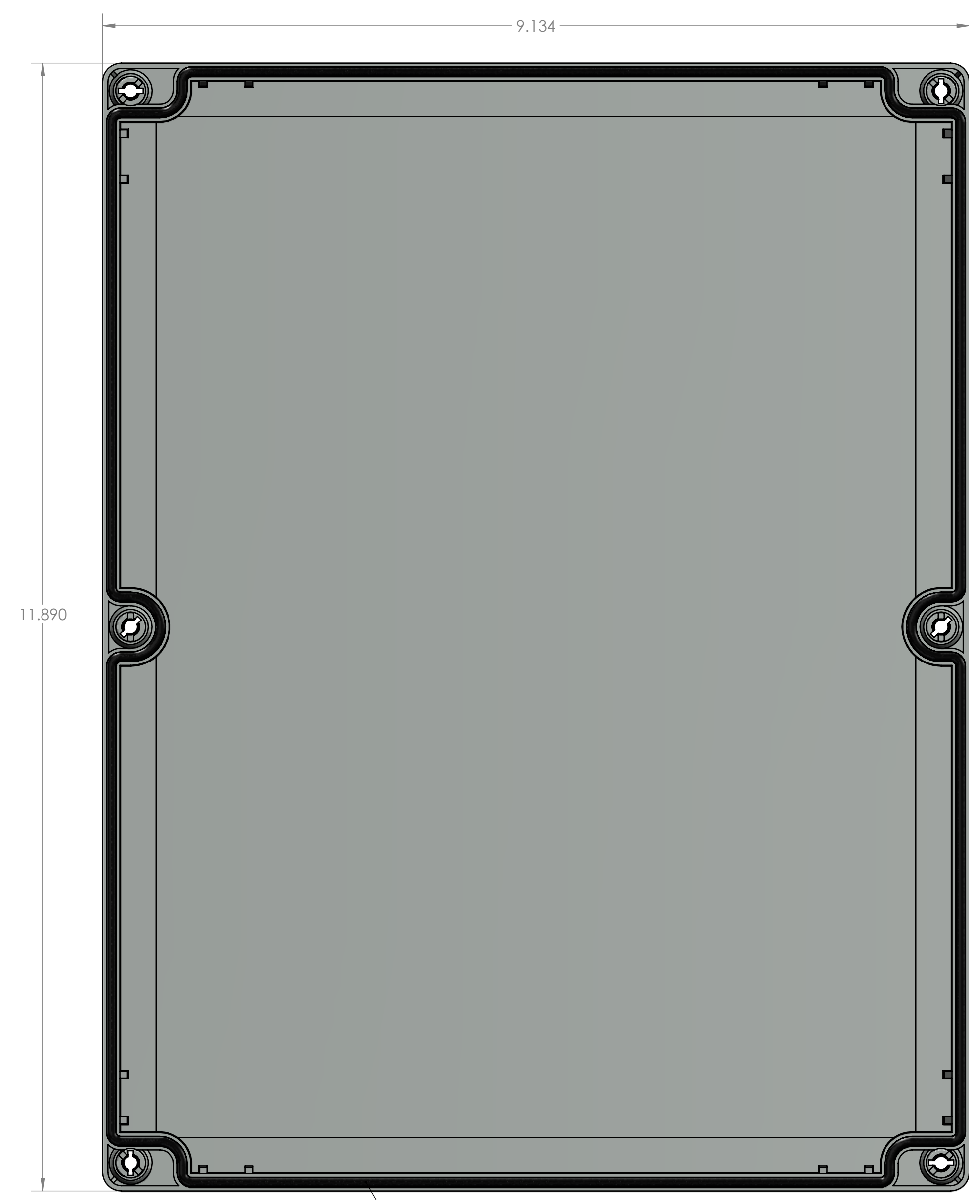
POLYURETHANE GASKET
