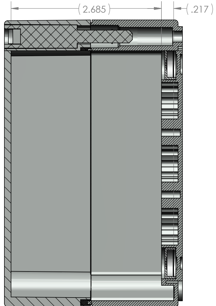
SECTION B-B
